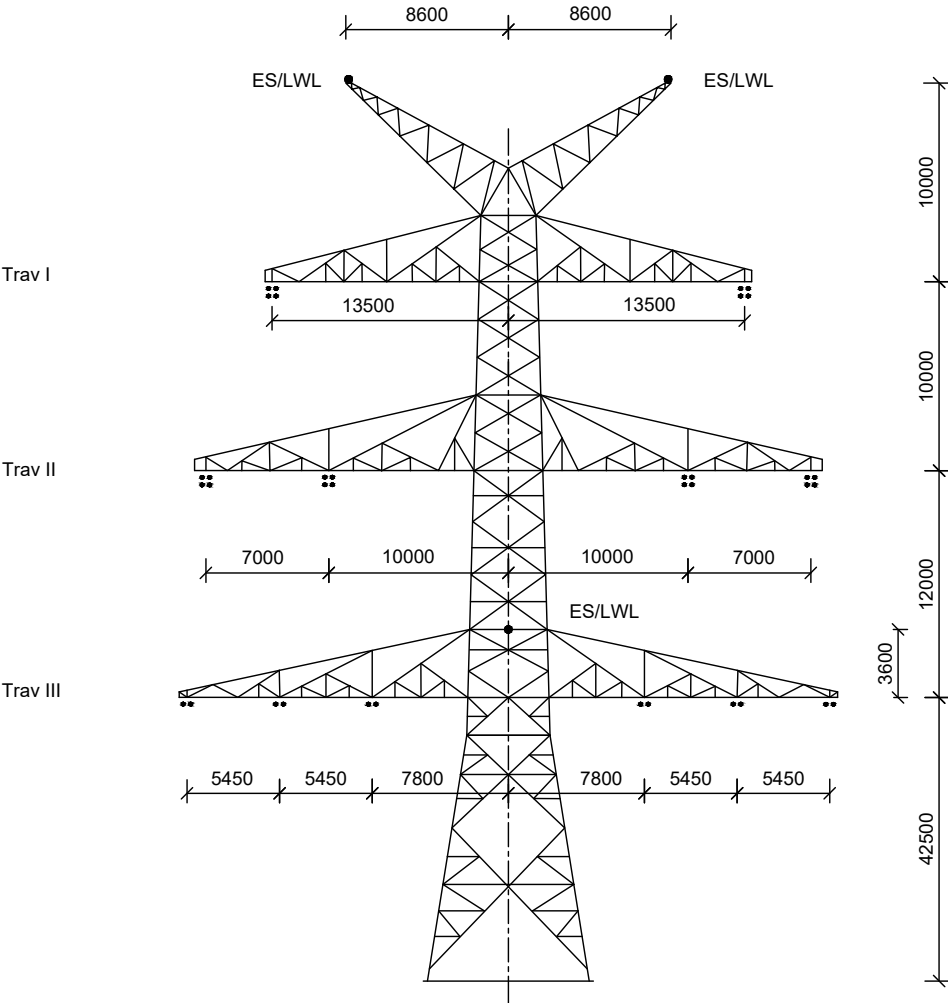
WA120-39.00 (+3.5m SFE) B175: Mast Nr. 6A
